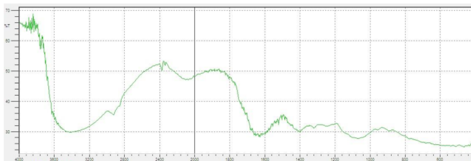
Figure 2 . FTIR spectra of A. manihot from Kotamobagu
