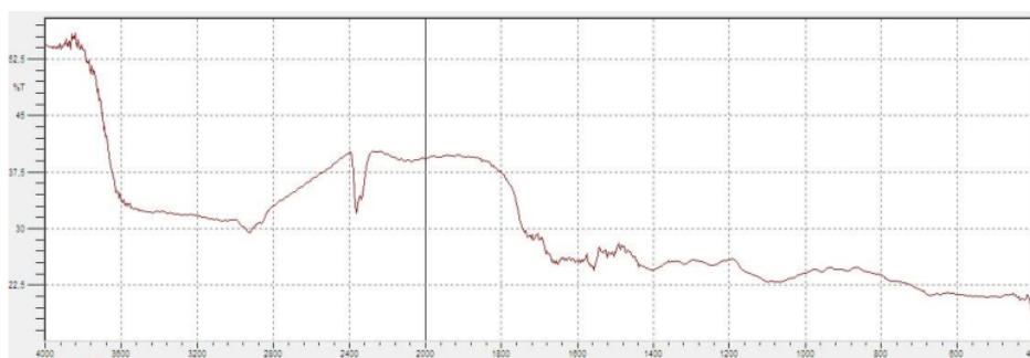
Figure 3 . FTIR spectra of A. manihot from Tomohon
