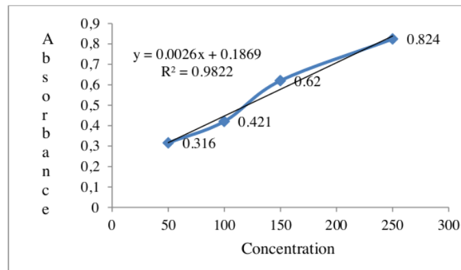
Figure 1 . Standard curve of quercetine for total flavonoid
